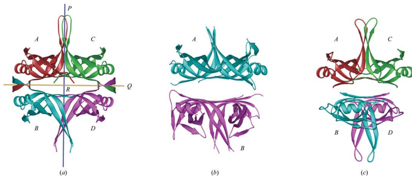
Figure 3 The quaternary structure of MsSSB ( a ) along with those of DrSSB ( b ) and EcSSB ( c ). While MsSSB and EcSSB are tetramers, DrSSB is a dimer, with each monomer made up of two OB-fold domains. The three perpendicular twofold axes P , Q and R , which relate the subunits of the MsSSB tetramer, are depicted.
