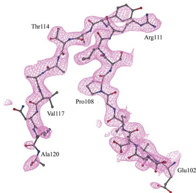
Figure 1 A 2F_o - F_c omit map for the stretch of residues 102–120. The figure was generated using BOBSCRIPT (Esnouf, 1997). The map was contoured at 1\sigma .
